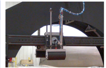
Fully enclosed wrap zone for more protection
