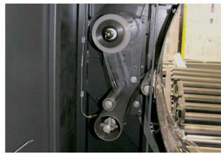
Automatic cutting/clamping finger safe unit
