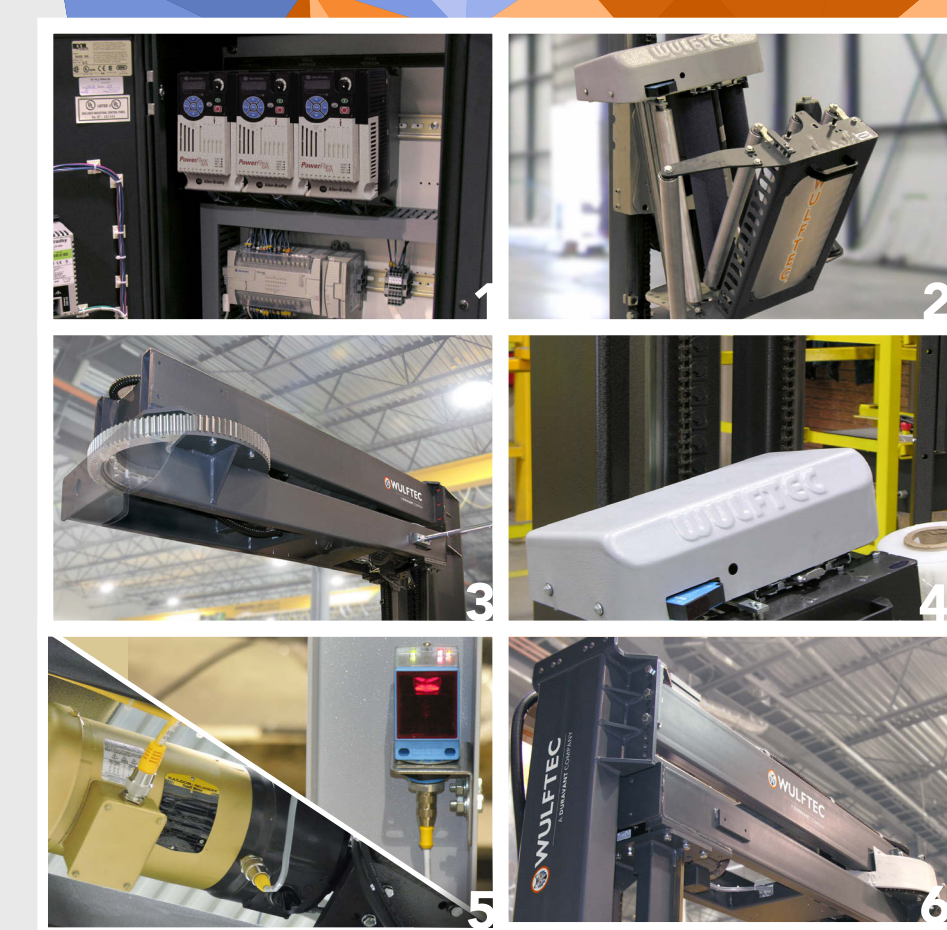
WRT-150 WITH SCALE
